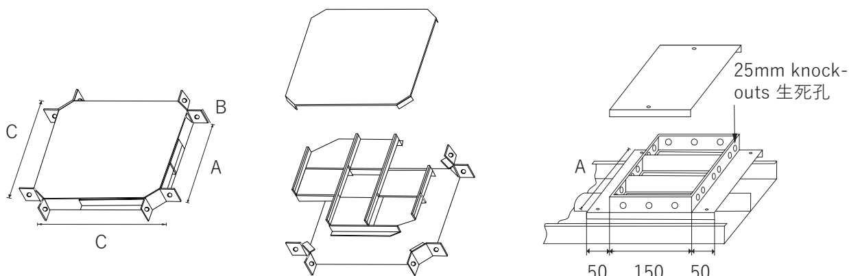
Junction Box 線槽過路箱
