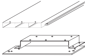
A type (Sealed Lid 密封蓋)
