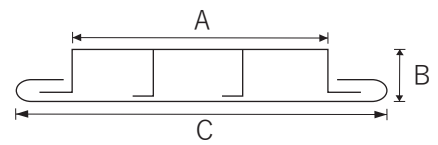
3-compartment type 3 倉型
